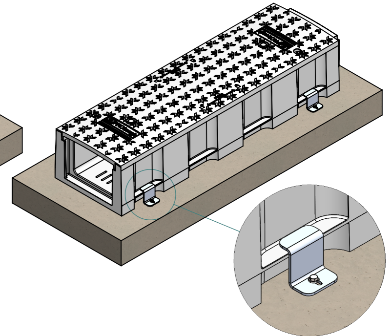
DETAIL D
